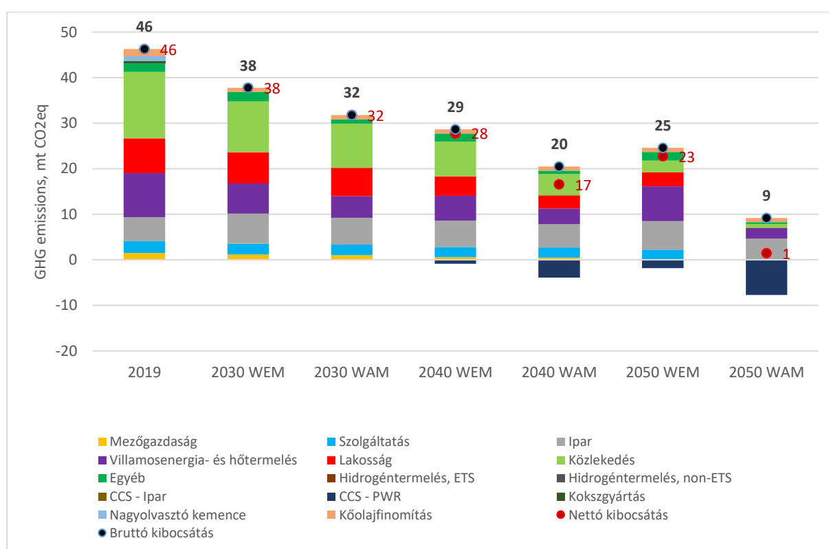
89Figure – Projected evolution of greenhouse gas emissions by sector , WEM and WAM scenarios (2019-2050, mt CO 2 e/year) Source: Fact 1: Eurostat, forecast: REKK
