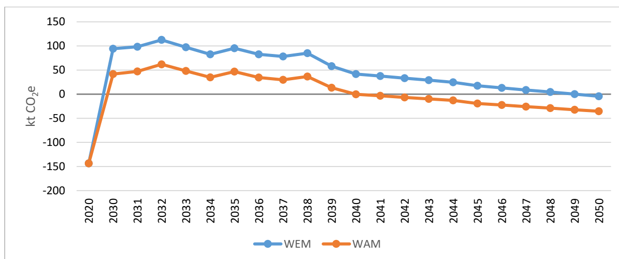
112Figure - Figure 3 GHG emissions of the LULUC sector according to WEM and WAM projections (2020-2050) Source: WHO
