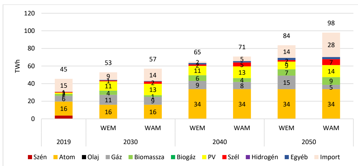
91Figure – Expected evolution of electricity generation, consumption and imports under the WEM and WAM scenarios (2019-2050, TWh/year) Source: Facts: Eurostat, Forecast: REKK
