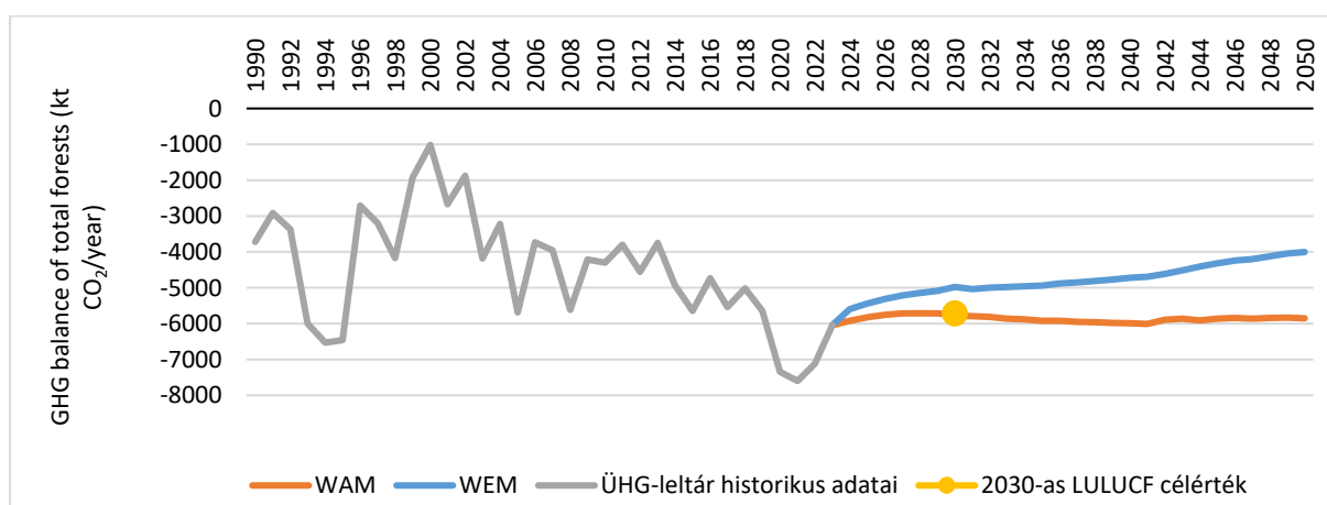
113Figure - Matching GHG inventory data with projection curves and 2030 target Source: SOE
