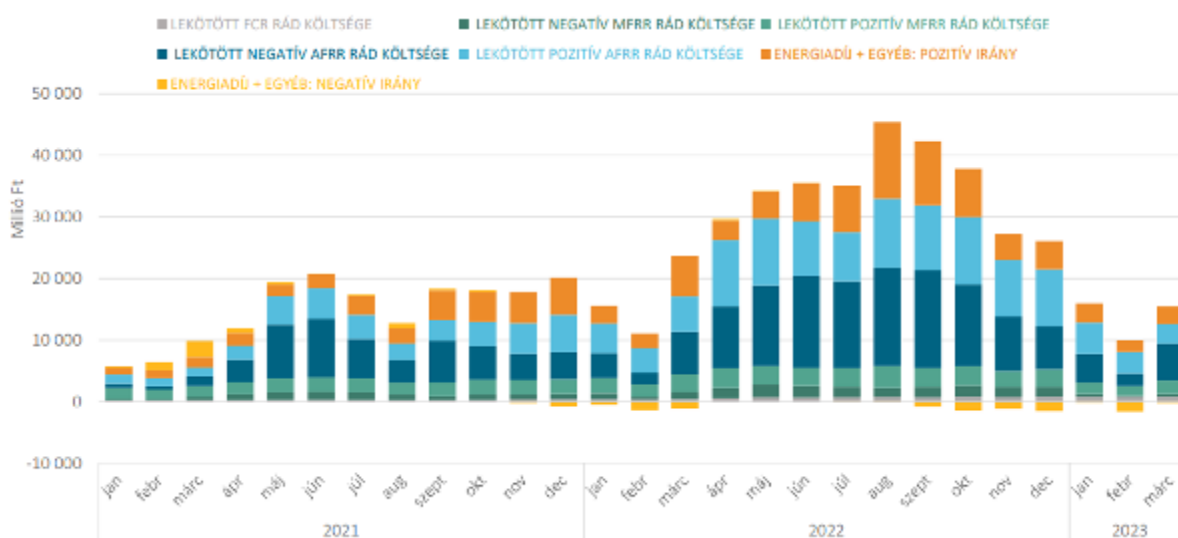
72Figure – Total cost of regulation used by the electricity system operator (2021-2023) Source - MEKH monthly report
