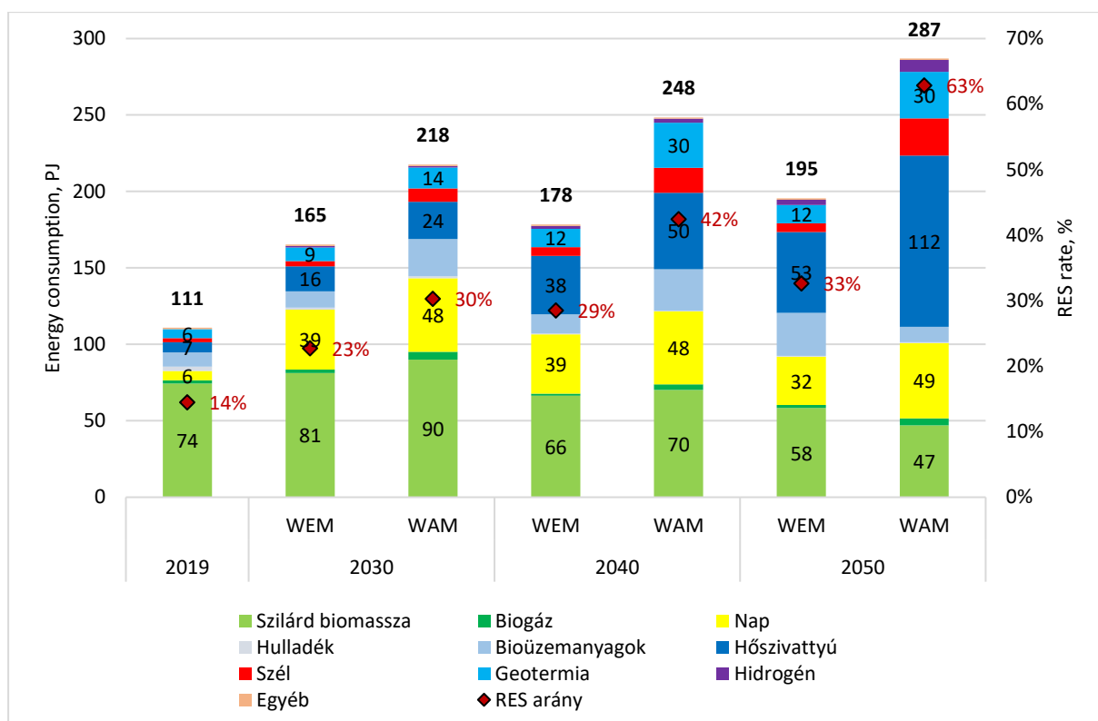
95Figure – Renewable energy use by source, WEM and WAM scenarios (2019-2050, PJ/year) Source: Fact 1: Eurostat, forecast: REKK
