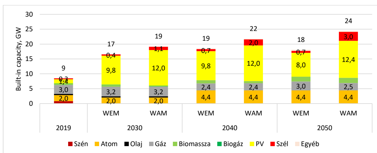
90Figure – Expected evolution of installed electricity generation capacity under the WEM and WAM scenarios (2019-2050, GW) Source: Fact 1: Eurostat, forecast: REKK
