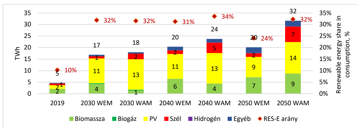
97Figure – Renewable electricity generation (TWh) and renewable electricity share in consumption (RES-E, %), WEM and WAM scenarios (2019-2050) Source: Fact 1: Eurostat, forecast: REKK
