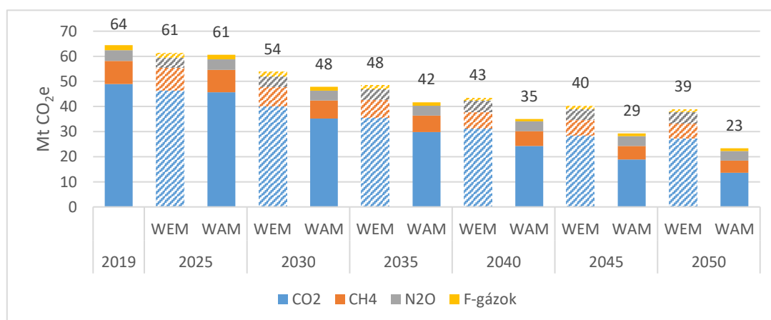
88Figure – Expected evolution of net greenhouse gas emissions by gas (2019-2050, Mt CO 2 e/year) Source: Fact 1: Eurostat, forecast: REKK, AKI, HungaroMet
