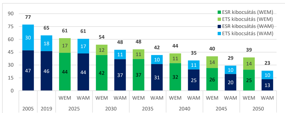
87Figure – Evolution of gross emissions in the ETS and ESS sectors (2005, 2019-2050, Mt CO 2 e/year) Source: Fact 1: Eurostat, forecast: REKK, AKI, HungaroMet
