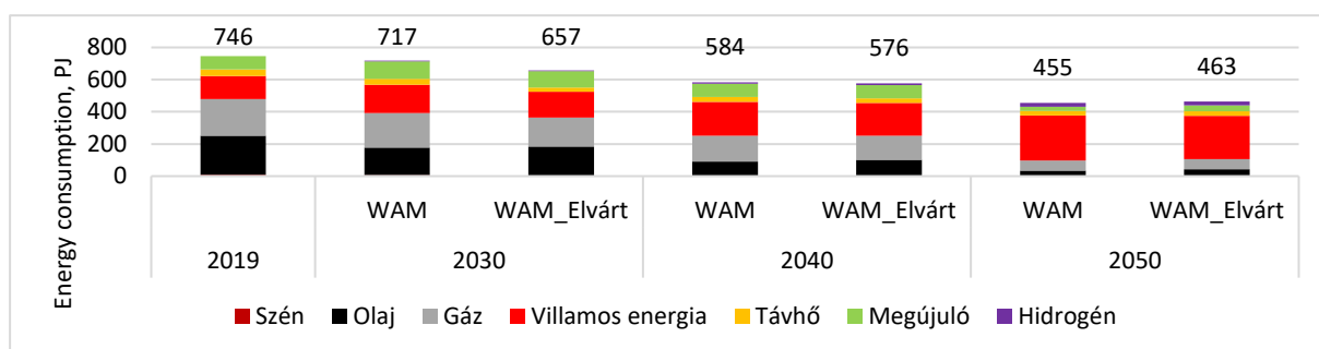
117Figure - Final energy consumption according to GAP analysis between set and expected targets (2019-2050, PJ) Source: REKK
