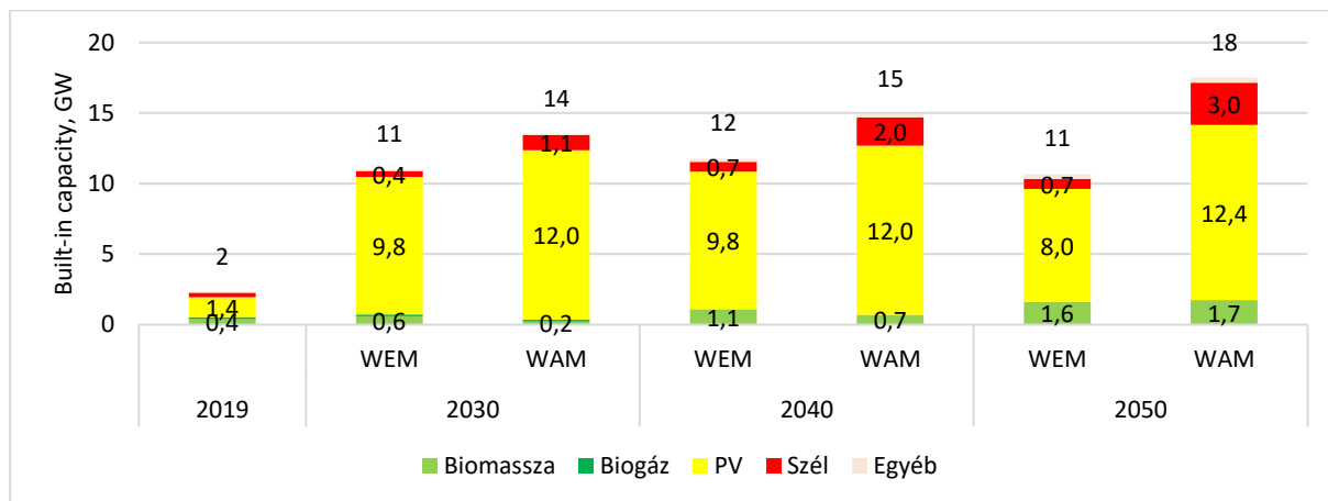
96Figure – Expected evolution of installed renewable capacity under the WEM and WAM scenarios (2019-2050, GW) Source: Fact 1: Eurostat, forecast: REKK
