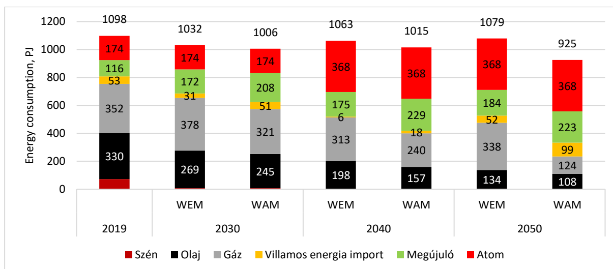
107Figure – Expected evolution of primary energy consumption, by fuel and its composition in the WEM and WAM scenarios – impact of new policy measures (2019-2050, PJ)
