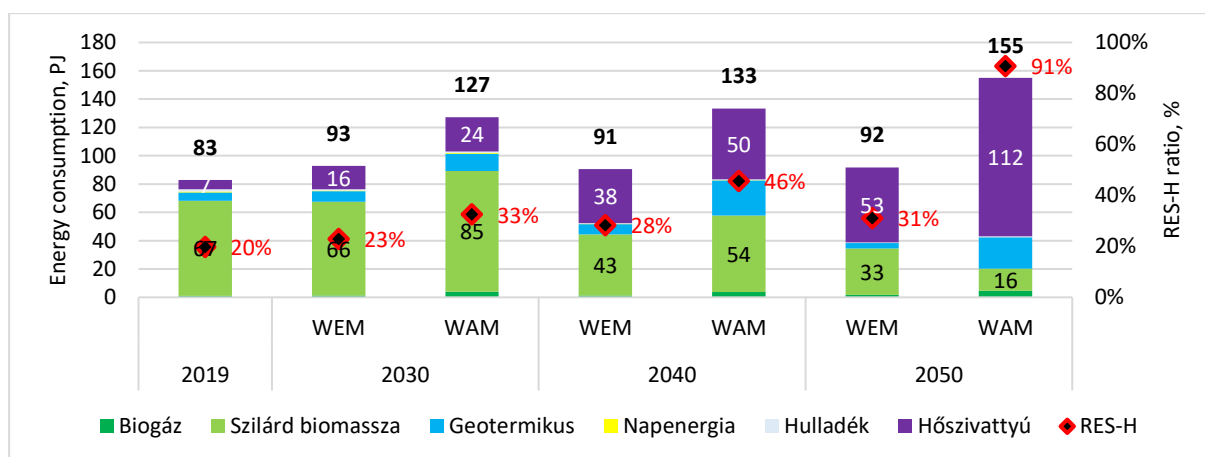
99Figure – Renewable energy use in the heating and cooling sector (PJ) and the renewable share (RES – H/C, %), WEM and WAM scenarios (2019-2050) Source: Fact 1: Eurostat, forecast: REKK
