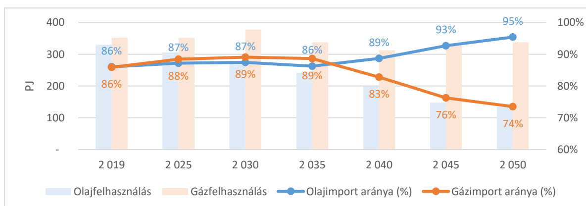
53Figure – Primary energy consumption (PJ) and net imports (%) of natural gas and oil, WEM scenario (2019-2050)
