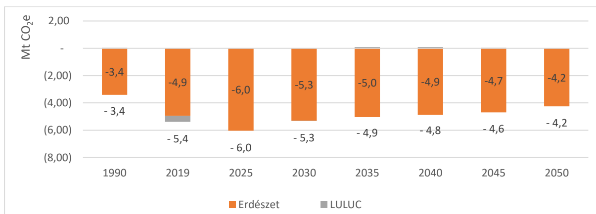
22Figure - Net GHG removals of the LULUCF sector under the WEM scenario, 1990-2050 (Mt CO 2 e) Source: AKI, SOE ERTI, Eurostat
