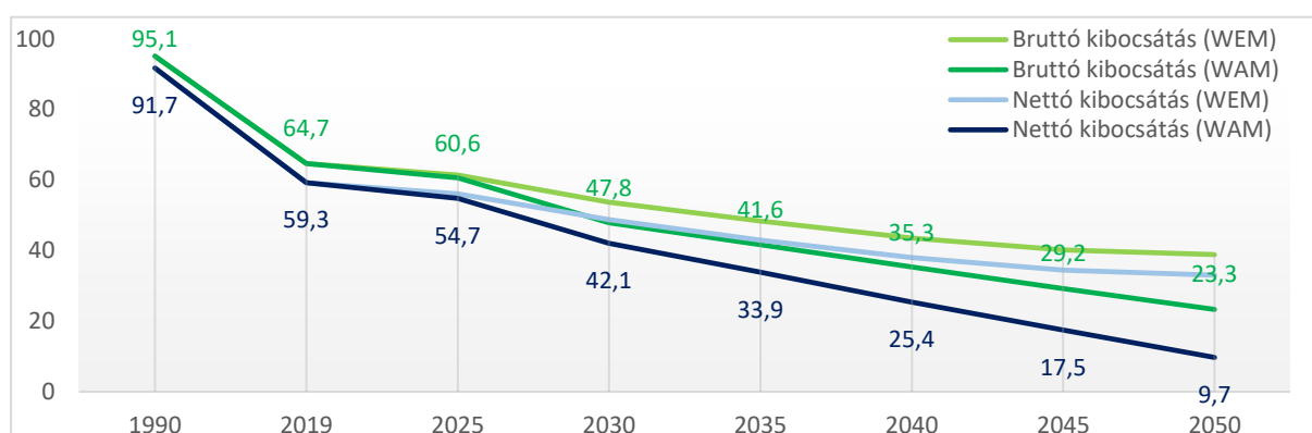
86Figure – Projected evolution of gross and net greenhouse gas emissions (1990, 2019-2050, Mt CO 2 e/year) Source:
