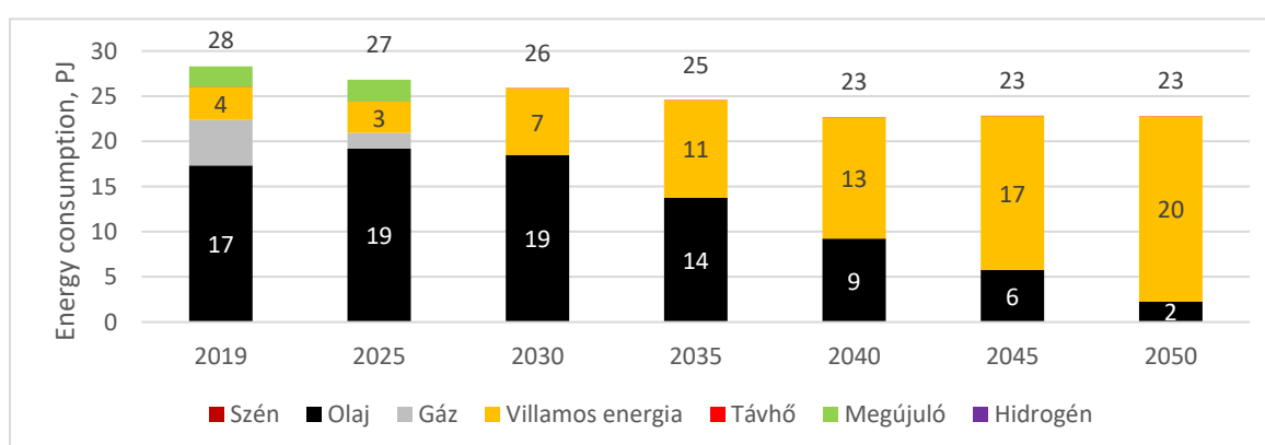
47Figure – Evolution of the fuel composition of energy use in the agricultural sector, WEM scenario (2019-2050, PJ/year)
